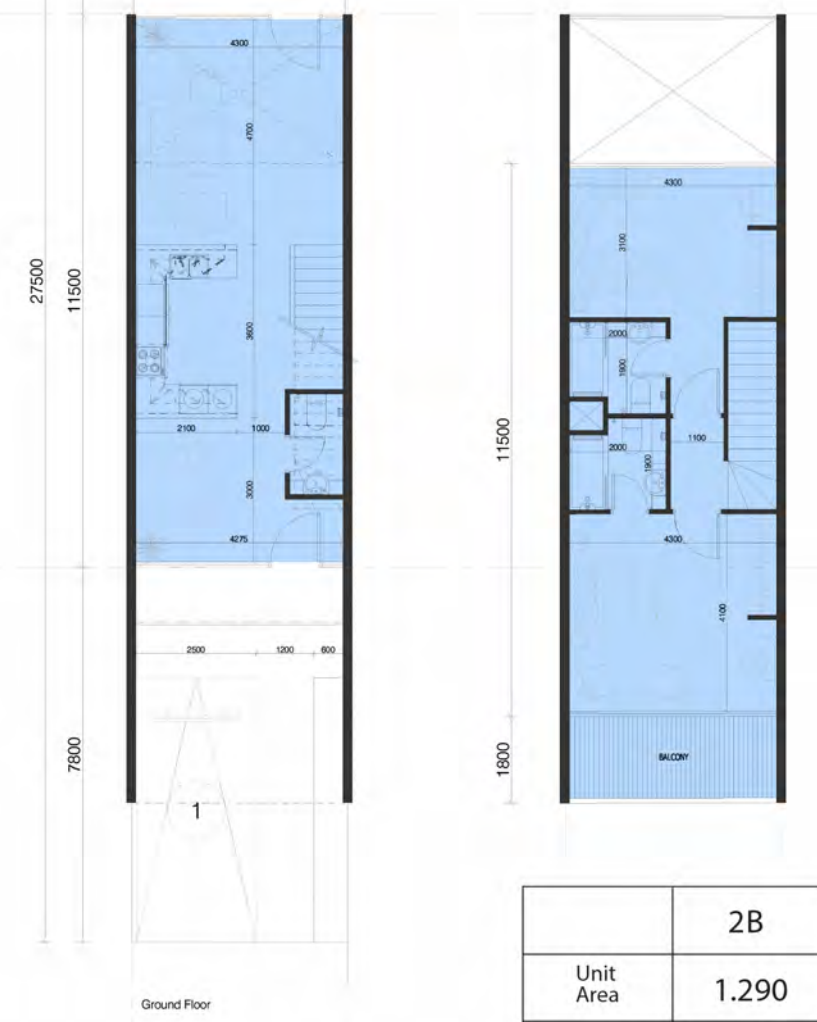
Ground Floor
