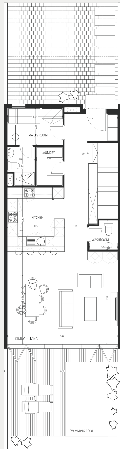
GROUND FLOOR
