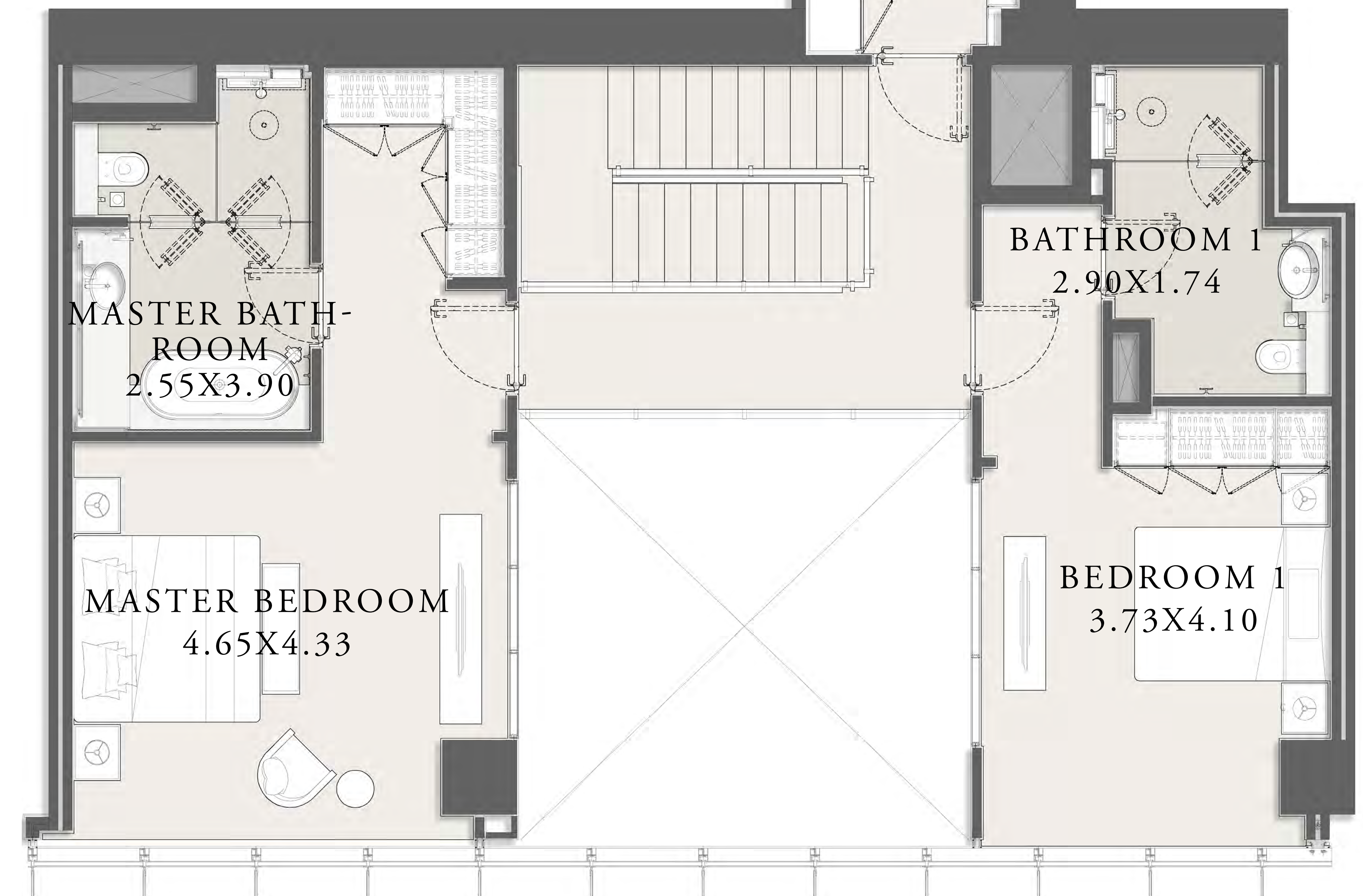
UPPER LEVEL
