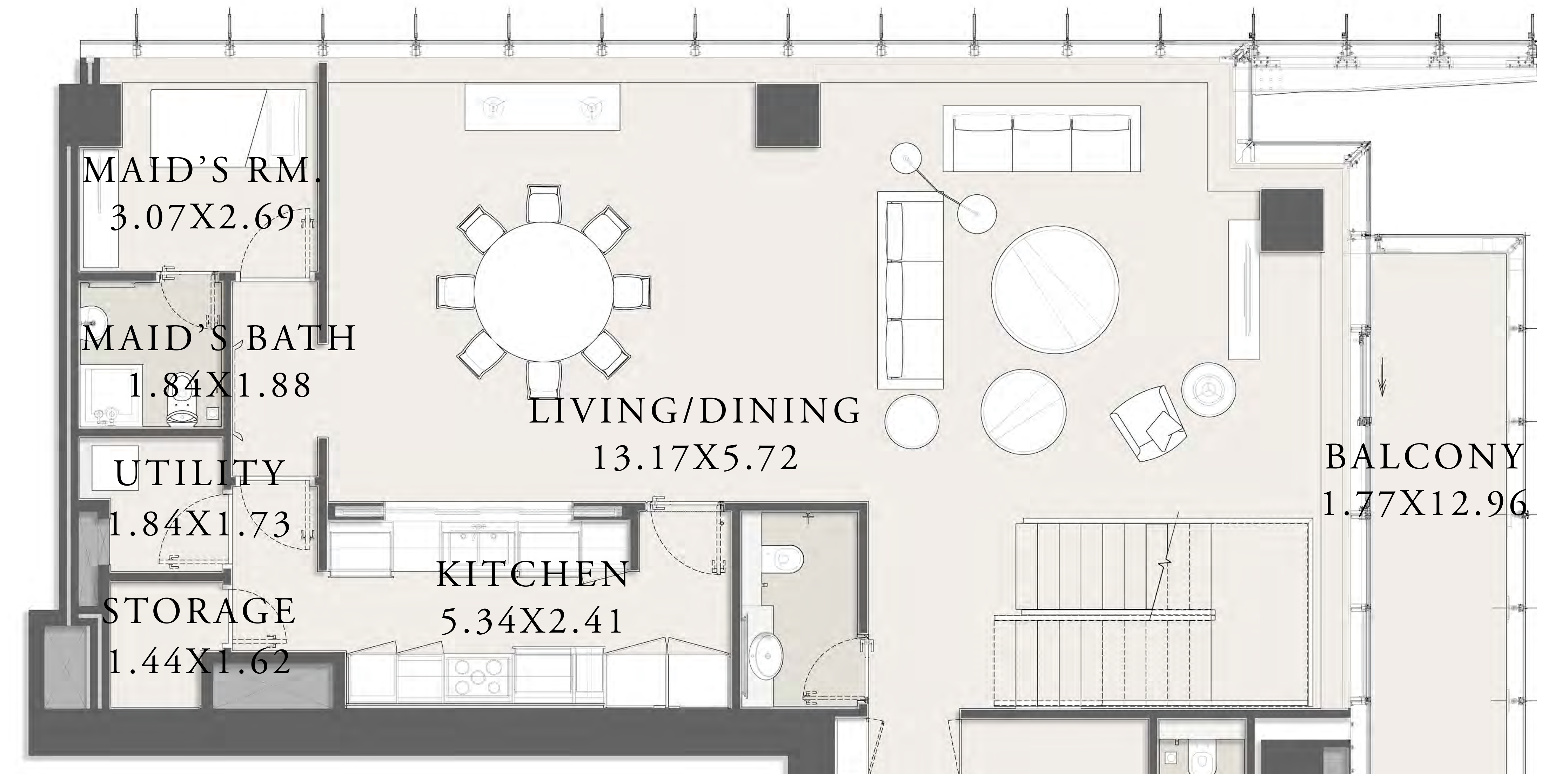
LOWER LEVEL
