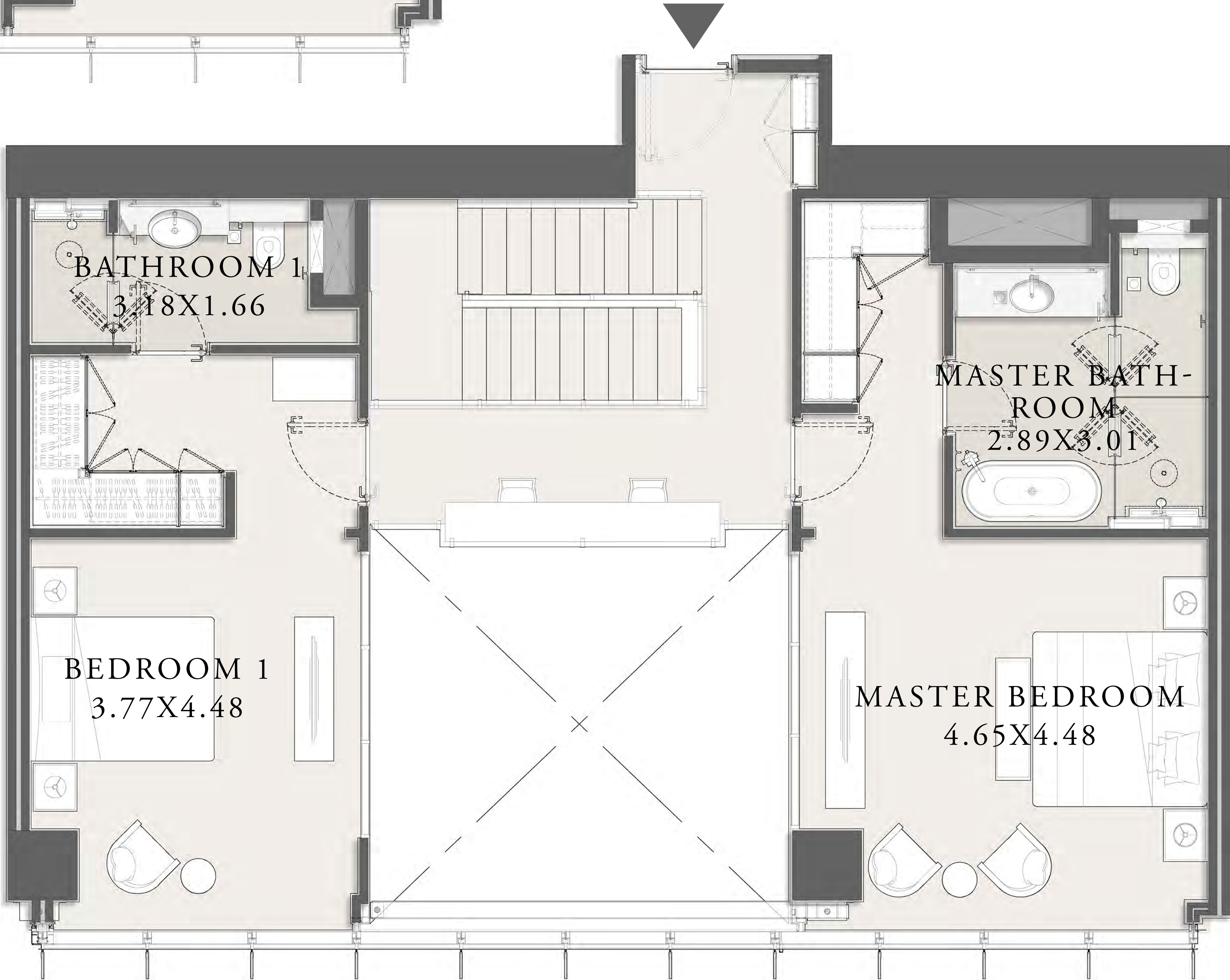
UPPER LEVEL
