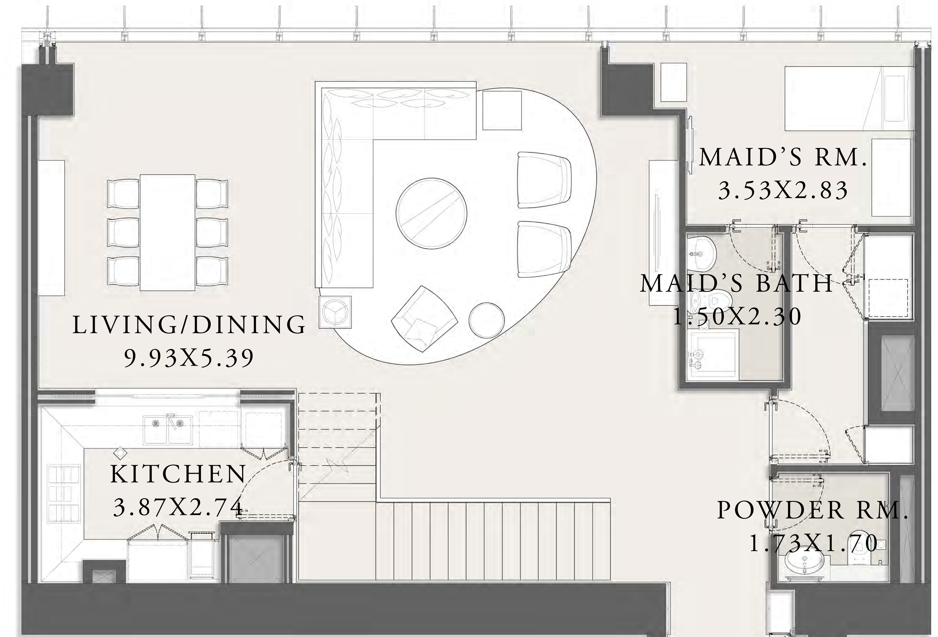
LOWER LEVEL
