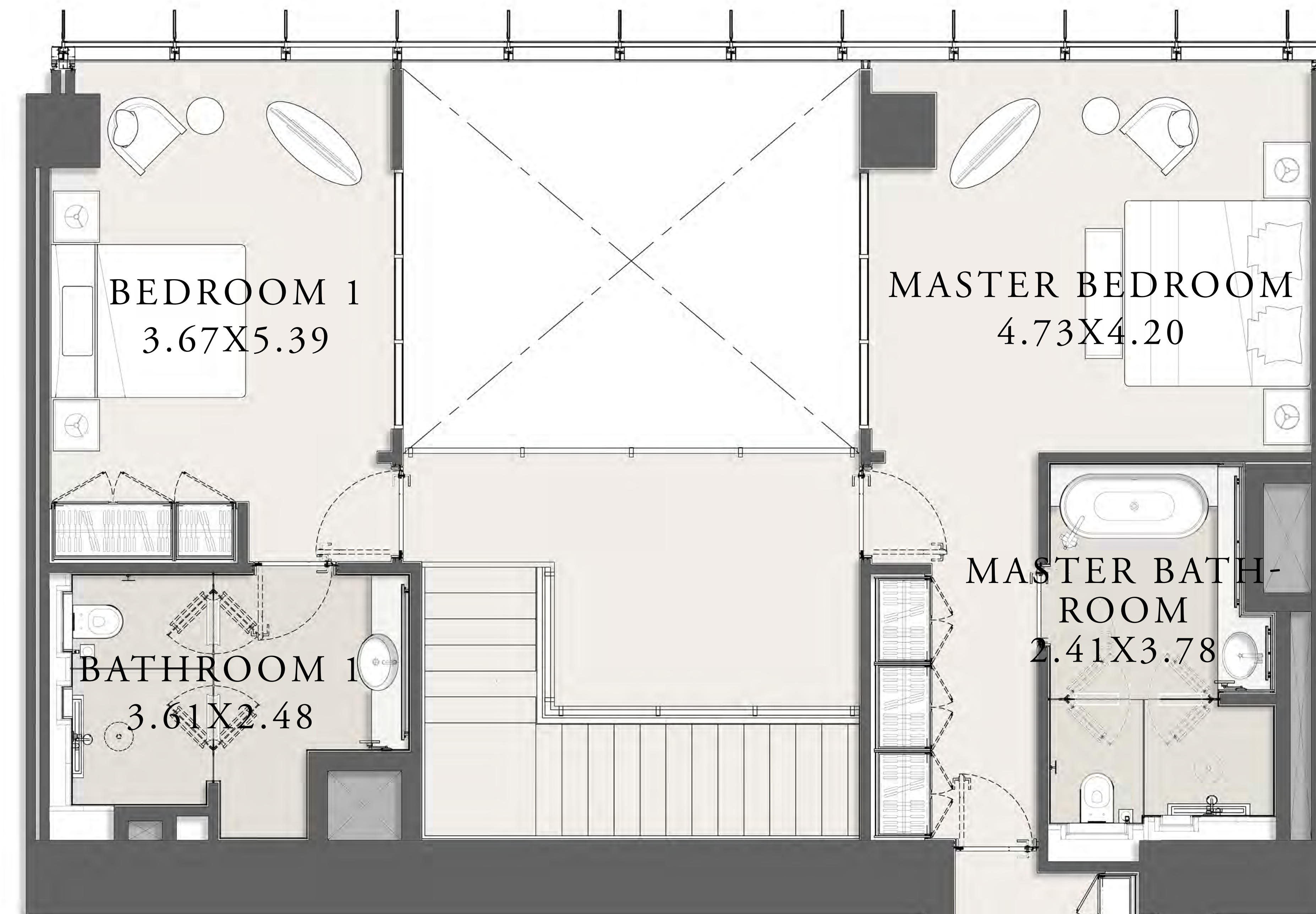
UPPER LEVEL
