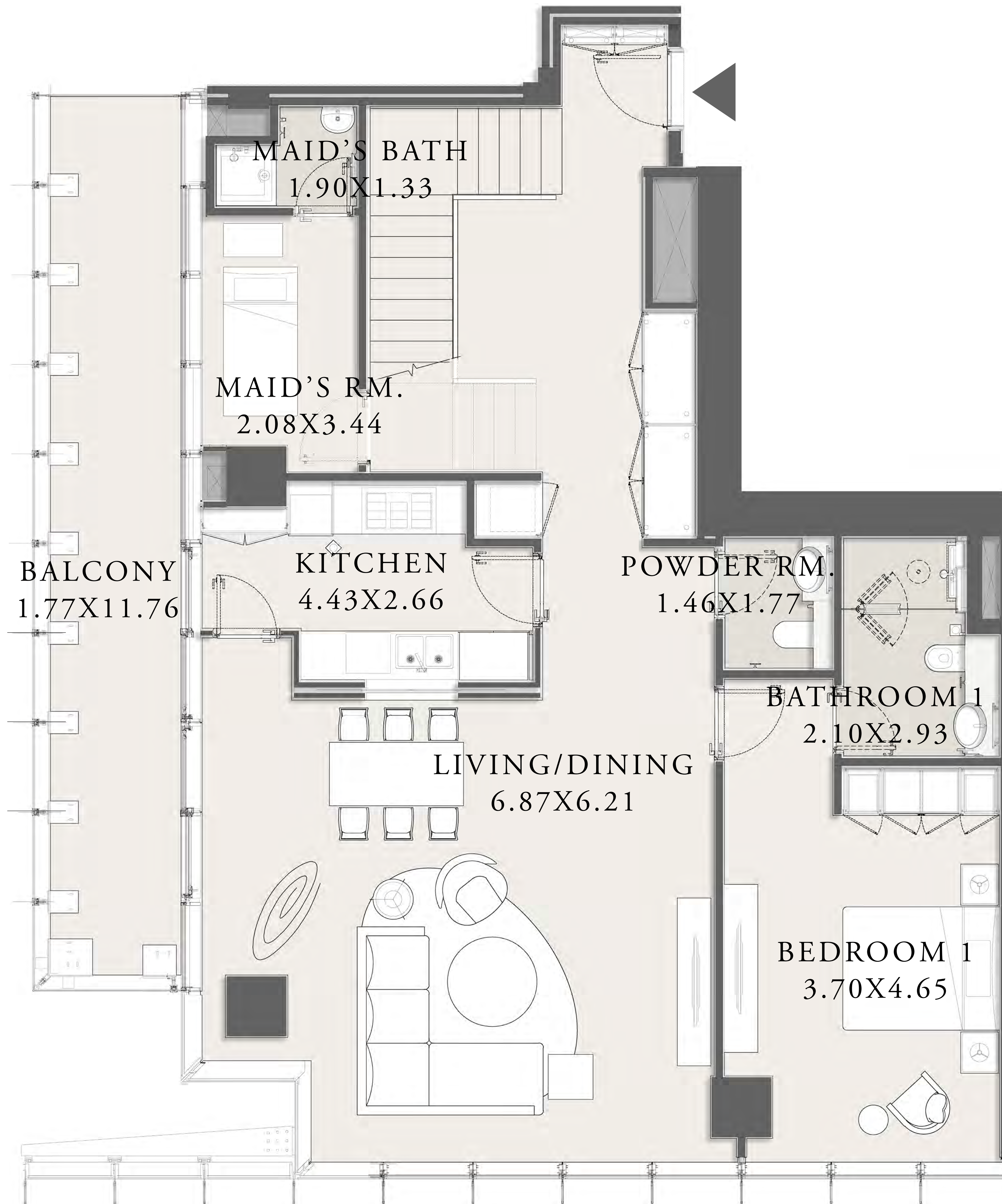
LOWER LEVEL
