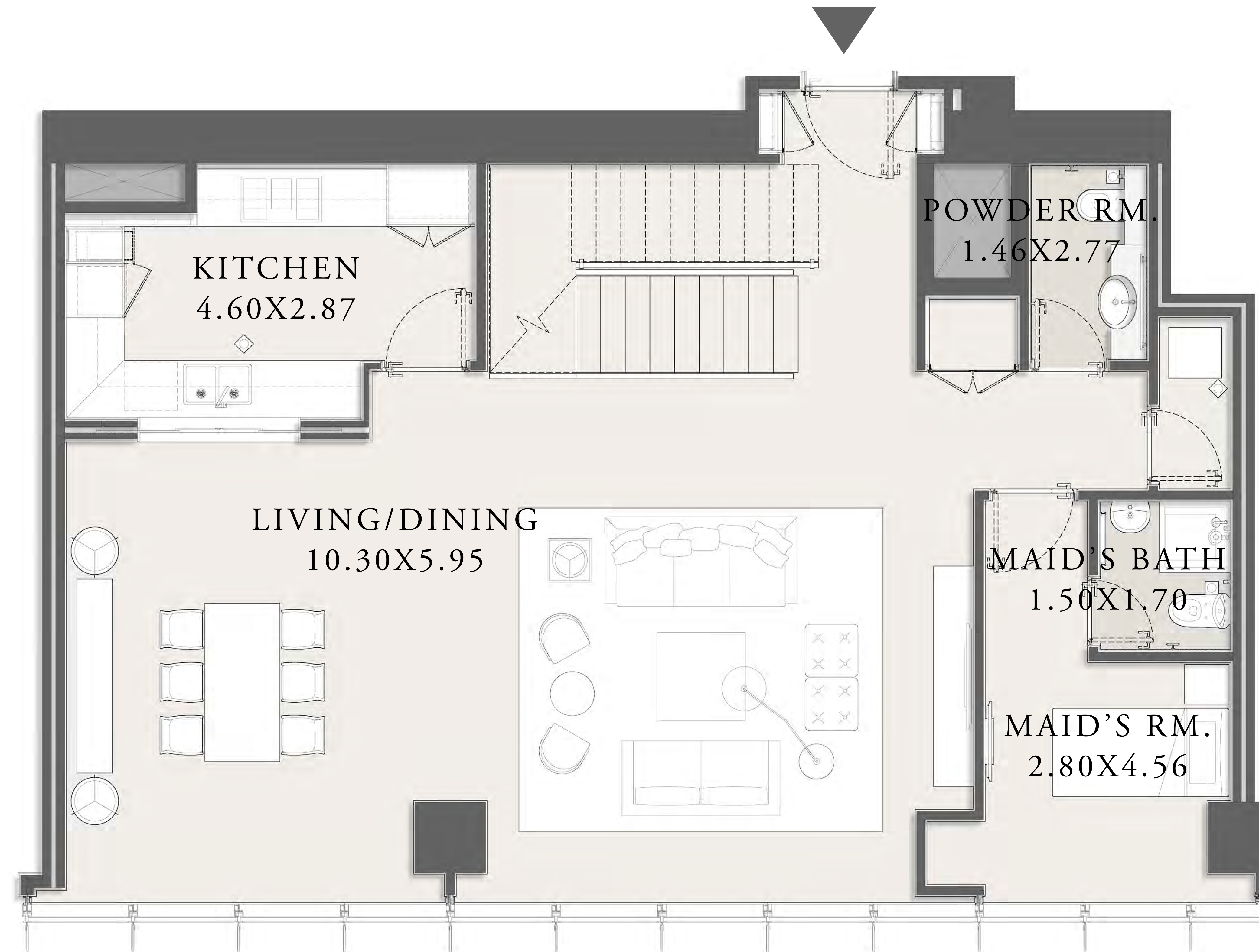
LOWER LEVEL
