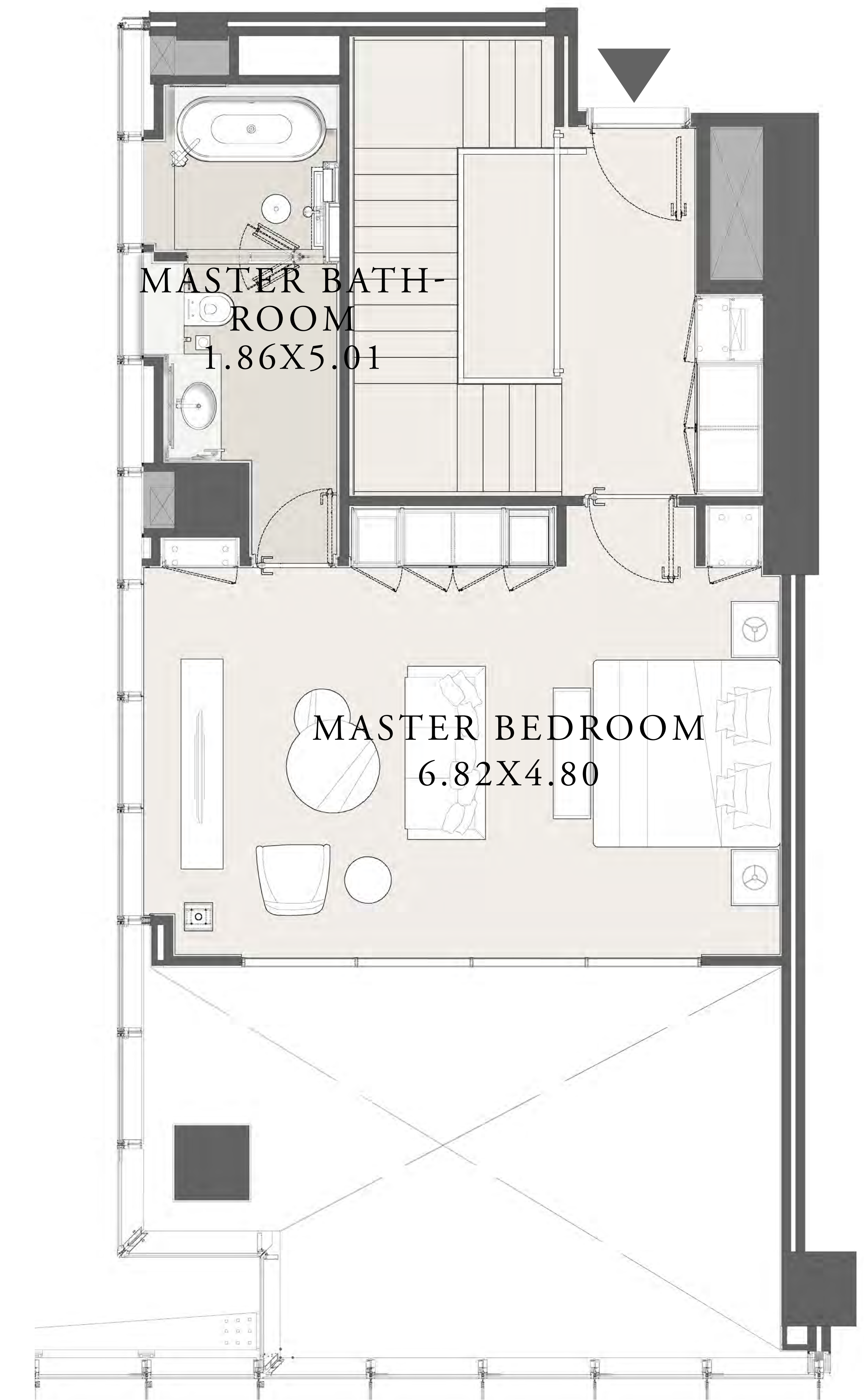
UPPER LEVEL
